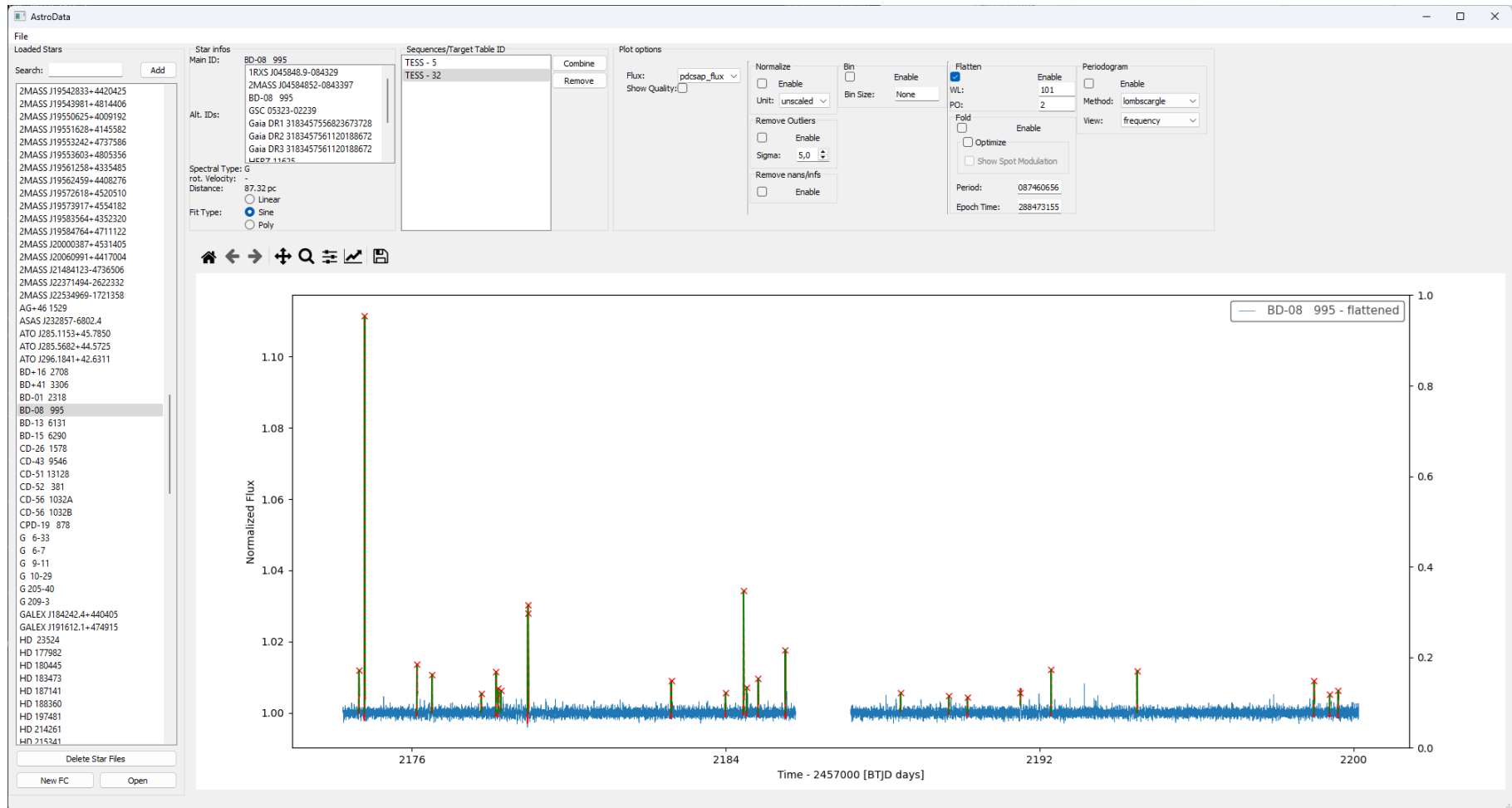
Fig. 2.5.: Main GUI window. Showing the same lightcurve as figure 2.2, with the difference that it is now flattened. The green line shows a fit of the flare. This is described in chapter 3.2.
