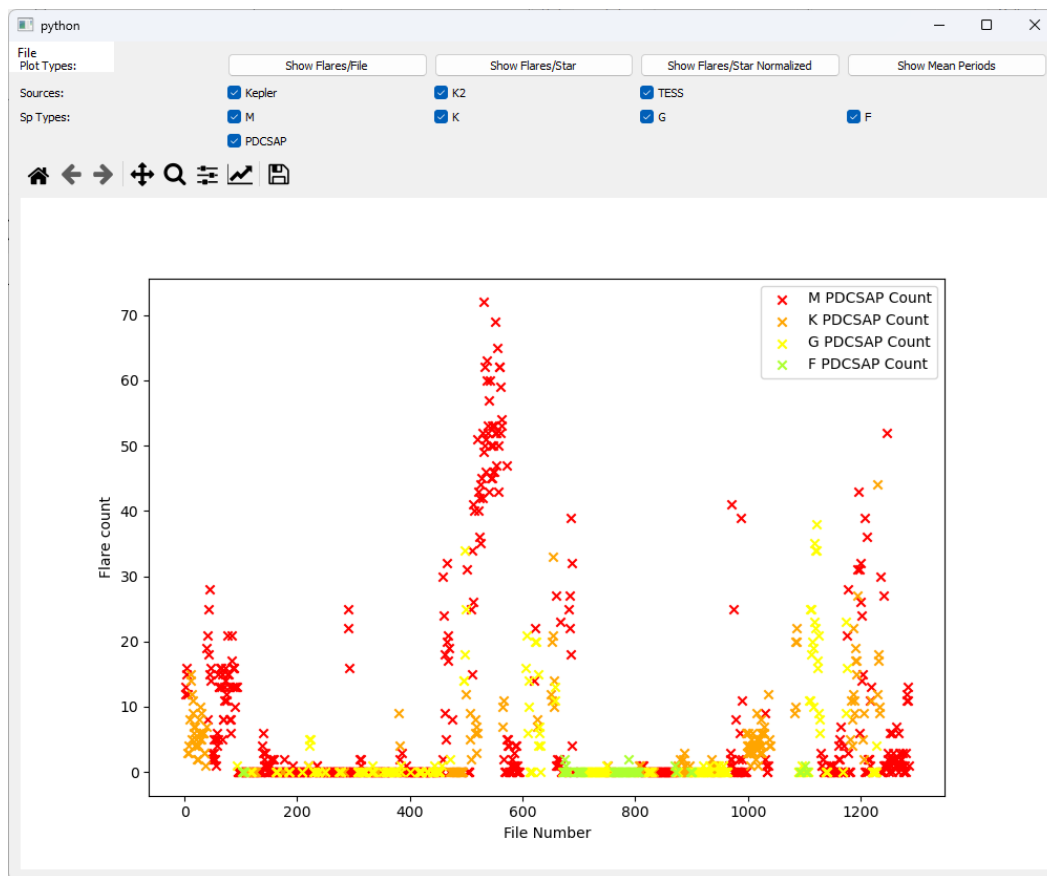
Fig. 2.9.: Debugging statistics window. Has the option to filter data by sources and spectral type for Kepler/K2/TESS pdcsap flux data. It has the ability to show various statistics like flares per fits file, flares per star (total or normalized to a period of 7 days), or the mean period detected. Plot showing statistics for "Show Flares/File".
