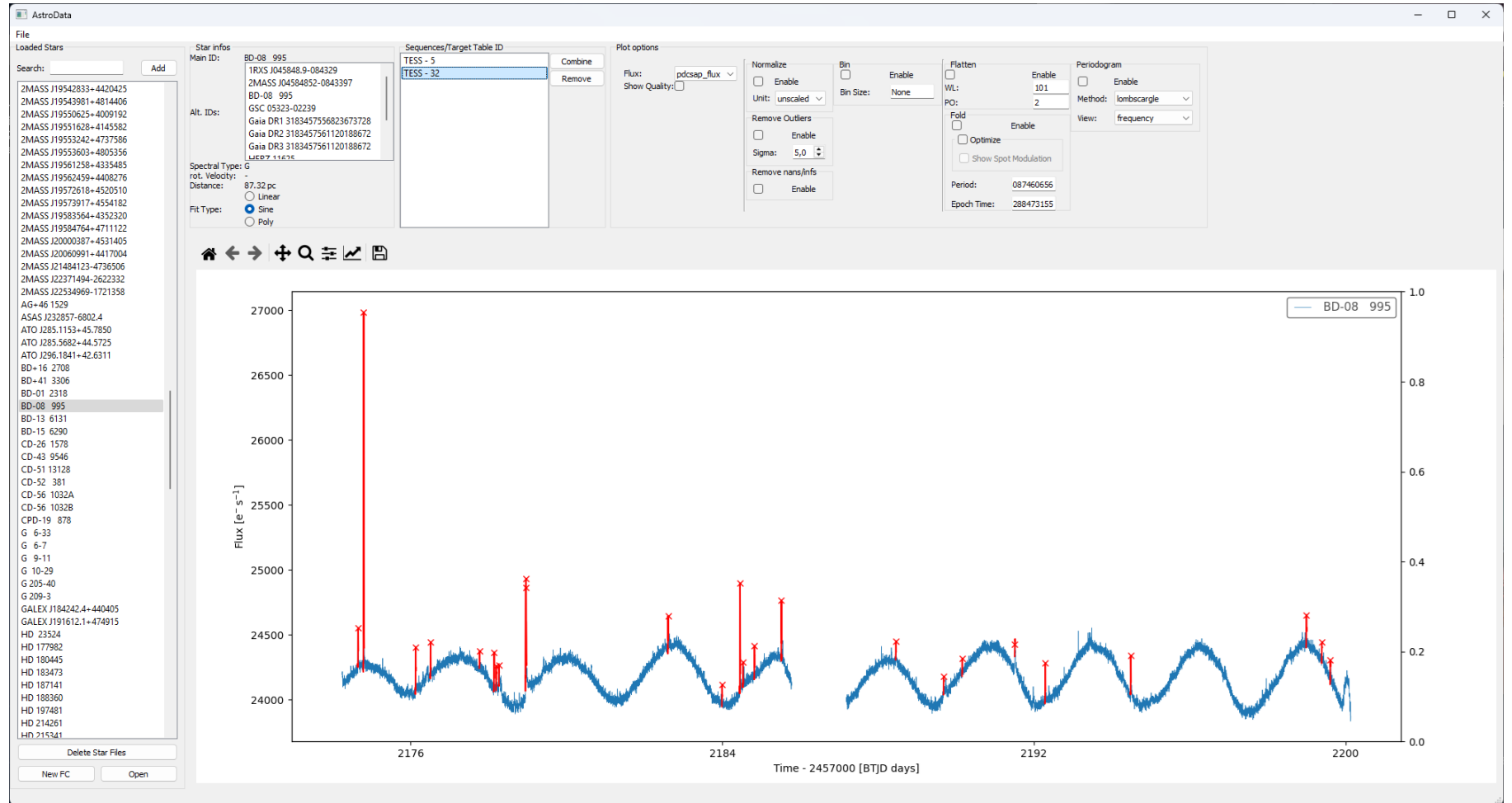
Fig. 2.2.: Main GUI window. This window was designed with the Qt5 designer shipped with PyQt5 (Riverbank Computing Limited (2025)). It shows a list of all available stars with their main identifier (taken from SIMBAD) sorted alphabetically. The "Star infos" box contains additional information on the star gathered from SIMBAD. The "Sequences/Target Table ID" box shows the list of all available lightcurves for the selected star, with an option to combine multiple to plot at once. To the right of the list of available lightcurves are different plot options, which utilize the different capabilities of the lightcurve python package (Lightcurve Collaboration et al. (2018)). In this image the TESS Sector 32 lightcurve of BD – 08 995 is shown. The red crosses show the peaks of the found flares, while the red overall over the lightcurve indicates the duration estimate of the flare.
