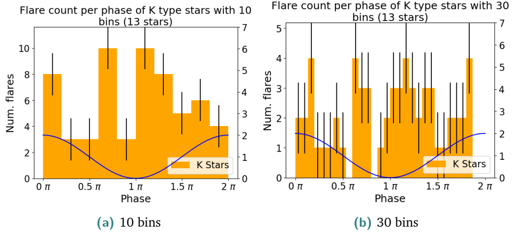
Fig. 4.7.: Histograms showing the number of flares with a normalized peak of greater than 1.05 per phase of 13 K dwarfs for which such flares could be detected. The x-axis represents the normalized phase of the folded lightcurves. There are 10 (a)/30 (b) bins of the phase, showing the number of flares per bin. The error bar shows the standard deviation for the histogram. The blue line indicates an idealized phase (sine curve), with the maximum at phase 0\pi/2\pi and the minimum at phase 1\pi .
