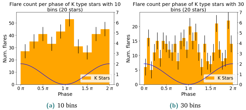
Fig. 4.8.: Histograms showing the number of flares with a normalized peak of less than 1.01 per phase of 20 K dwarfs for which such flares could be detected. The x-axis represents the normalized phase of the folded lightcurves. There are 10 (a)/30 (b) bins of the phase, showing the number of flares per bin. The error bar shows the standard deviation for the histogram. The blue line indicates an idealized phase (sine curve), with the maximum at phase 0\pi/2\pi and the minimum at phase 1\pi .
