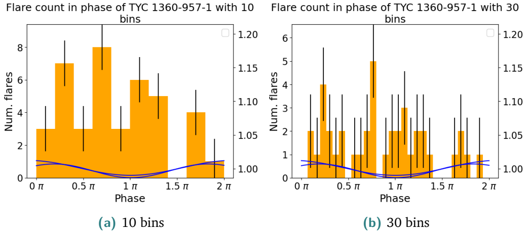
Fig. 4.18.: Histograms of TYC 1360-957-1 across the phase showing the number of flares in each bin. The error bars show the standard deviation for the histogram. The blue lines show the various fits for the folded lightcurves used to generate the data, with the phase minimum at 1\pi and phase maximum at 0\pi/2\pi .
