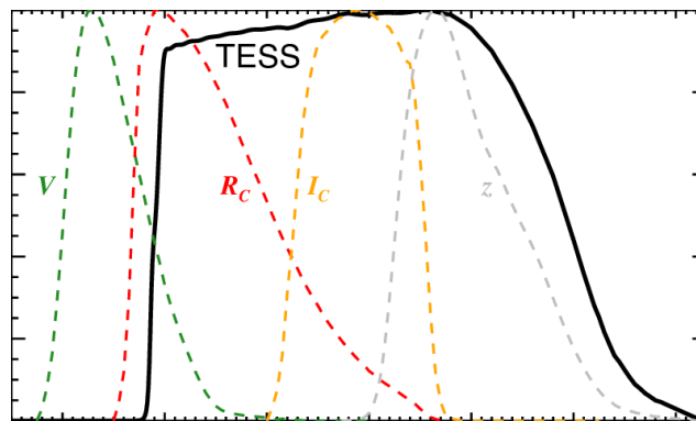
Fig. 1.5.: Image showing the Johnson V, R_C , I_C and SDSS z response curves and comparing it to TESS. Image from Rowe et al. (2009).
