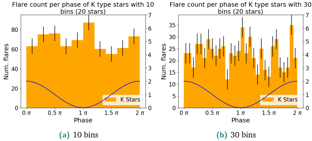
Fig. 4.9.: Histograms showing the number of flares with a normalized peak of less than 1.05 per phase of 20 K dwarfs for which such flares could be detected. The x-axis represents the normalized phase of the folded lightcurves. There are 10 (a)/30 (b) bins of the phase, showing the number of flares per bin. The error bar shows the standard deviation for the histogram. The blue line indicates an idealized phase (sine curve), with the maximum at phase 0\pi/2\pi and the minimum at phase 1\pi .
