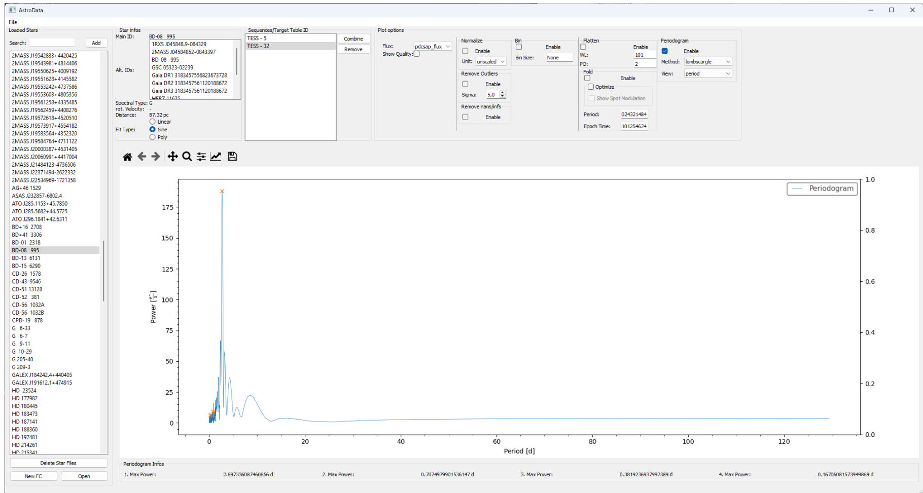
Fig. 2.7.: Main GUI window. Showing the periodogram of the lightcurve in figure 2.2 using the lombscargle algorithm. Furthermore it shows the four highest peaks (which are atleast 100 datapoints separated). The method is explained in chapter 3.2.
