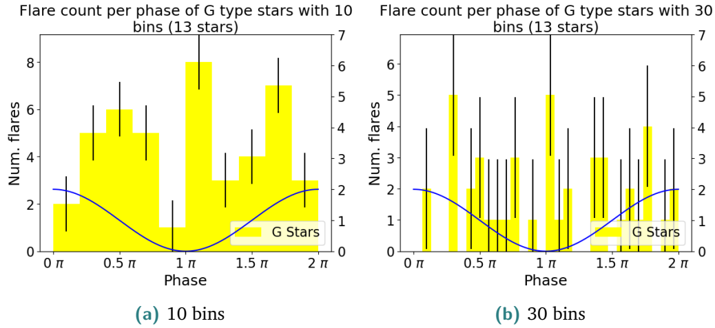
Fig. 4.12.: Histograms showing the number of flares with a normalized peak of greater than 1.05 per phase of 13 G dwarfs for which such flares could be detected. The x-axis represents the normalized phase of the folded lightcurves. There are 10 (a)/30 (b) bins of the phase, showing the number of flares per bin. The error bar shows the standard deviation for the histogram. The blue line indicates an idealized phase (sine curve), with the maximum at phase 0\pi/2\pi and the minimum at phase 1\pi .
