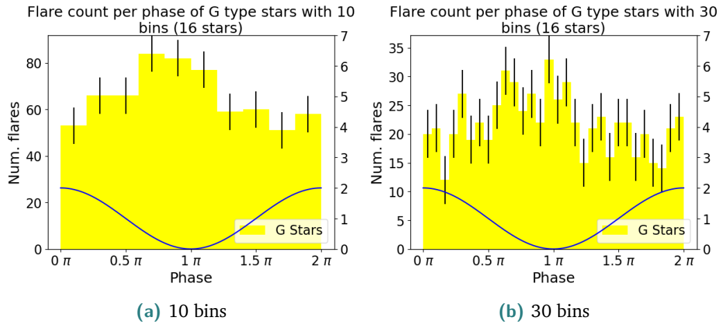
Fig. 4.11.: Histograms showing the number of flares with a normalized peak of less than 1.05 per phase of 16 G dwarfs for which such flares could be detected. The x-axis represents the normalized phase of the folded lightcurves. There are 10 (a)/30 (b) bins of the phase, showing the number of flares per bin. The error bar shows the standard deviation for the histogram. The blue line indicates an idealized phase (sine curve), with the maximum at phase 0\pi/2\pi and the minimum at phase 1\pi .
