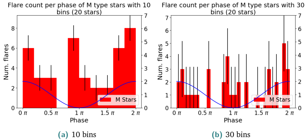
Fig. 4.3.: Histograms showing the number of flares with a normalized peak of greater than 1.5 per phase for 20 M dwarfs for which such flares could be detected. The x-axis represents the normalized phase of the folded lightcurves. There are 10 (a) /30 (b) bins of the phase, showing the number of flares per bin. The error bar shows the standard deviation for the histogram. The blue line indicates an idealized phase (sine curve), with the maximum at phase 0\pi/2\pi and the minimum at phase 1\pi .
