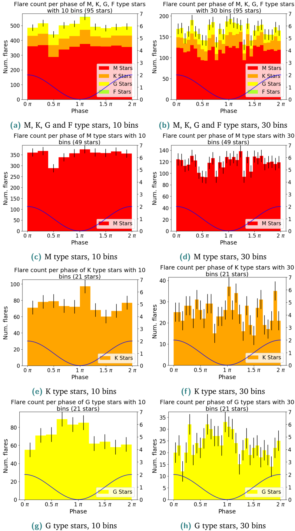
Fig. 4.14.: Histograms showing the number of flares per phase for all 95 dwarfs for which flares could be detected in panel a and b. Panel c to h show the histograms for spectral types M, K and G respectively as direct comparison. Otherwise same as previous figures.
