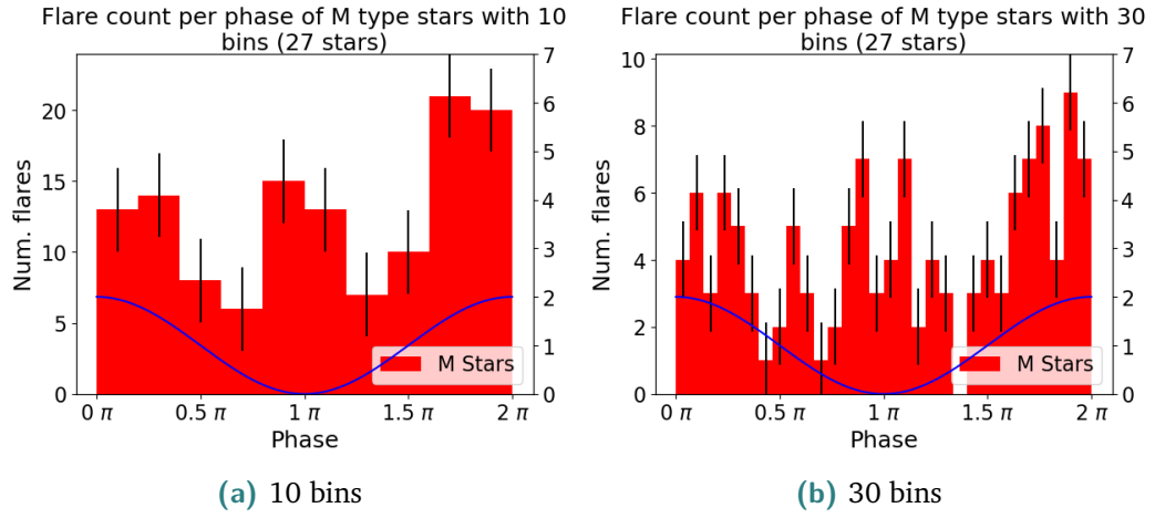
Fig. 4.2.: Histograms showing the number of flares with a normalized peak of greater than 1.25 per phase of 27 M dwarfs for which such flares could be detected. The x-axis represents the normalized phase of the folded lightcurves. There are 10 (a) /30 (b) bins of the phase, showing the number of flares per bin. The error bar shows the standard deviation for the histogram. The blue line indicates an idealized phase (sine curve), with the maximum at phase 0\pi/2\pi and the minimum at phase 1\pi .
