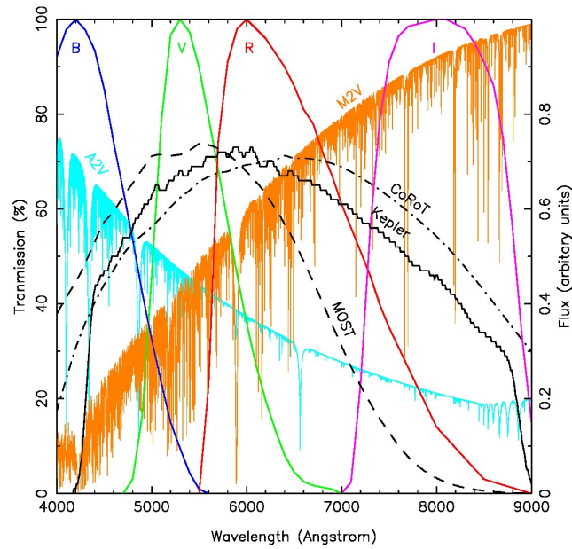
Fig. 1.4.: Image showing the Johnson B, V, R and I response curves and comparing it to the Kepler, MOST and CoRoT missions. Image from Rowe et al. (2009).
