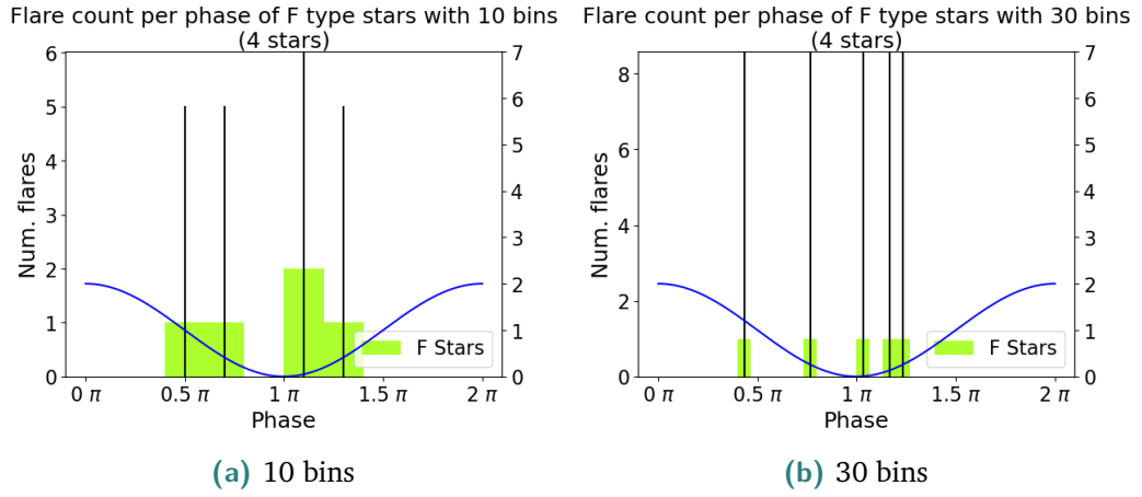
Fig. 4.13.: Histogram showing the number of flares per phase of 4 F dwarfs for which flares could be detected. The x-axis represents the normalized phase of the folded lightcurves. There are 10 bins (a)/30 bins (b) of the phase, showing the number of flares per bin. The error bar shows the standard deviation for the histogram. The blue line indicates an idealized phase (sine curve), with the maximum at phase 0\pi/2\pi and the minimum at phase 1\pi .
