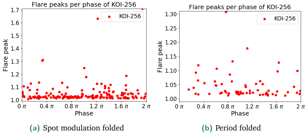
Fig. 4.33.: Distributions of flare peaks for KOI-256 in relation to the normalized phase at which they occurred. Y-Axis shows the flare peak and is limited to the value of the highest peak detected. The x-axis shows the normalized phase. Panel a flare peak distribution on the normalized phase for the detected spot modulation. Panel b shows the flare distribution for the detected rotational periods.
