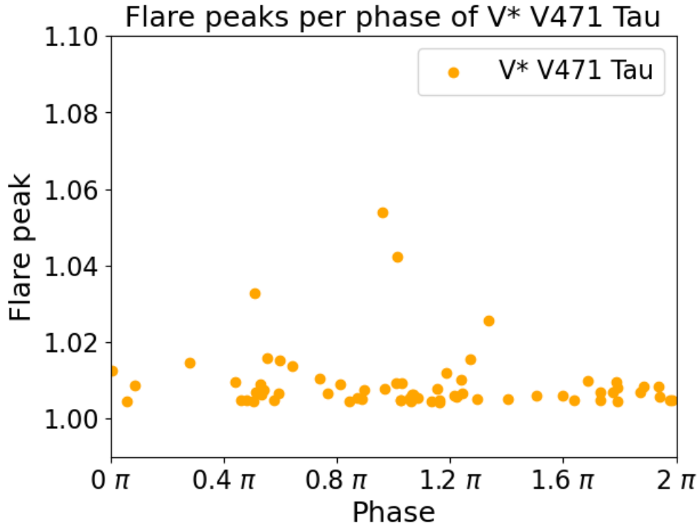
Fig. 4.25.: Distribution of flare peaks in relation to the normalized phase at which they occurred. Y-Axis shows the flare peak and is limited to the value of the highest peak detected. The x-axis shows the normalized phase.
