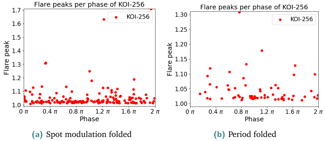
Fig. 4.33.: Distribution of flare peaks in relation to the normalized phase at which they occurred. Y-Axis shows the flare peak and is limited to the value of the highest peak detected. The x-axis shows the normalized phase.
