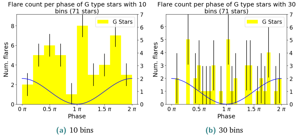
Fig. 4.12.: Histograms showing the amount of flares with a normalized peak of greater than 1.05 per phase for all 71 G dwarfs used in this study. The x-axis represents the normalized phase of the folded lightcurves. There are 10 (a)/30 (b) bins of the phase, showing the number of flares per bin. The error bar shows the standard deviation for the histogram. The blue line indicates an idealized phase (sine curve), with the maximum at phase 0\pi/2\pi and the minimum at phase 1\pi .
