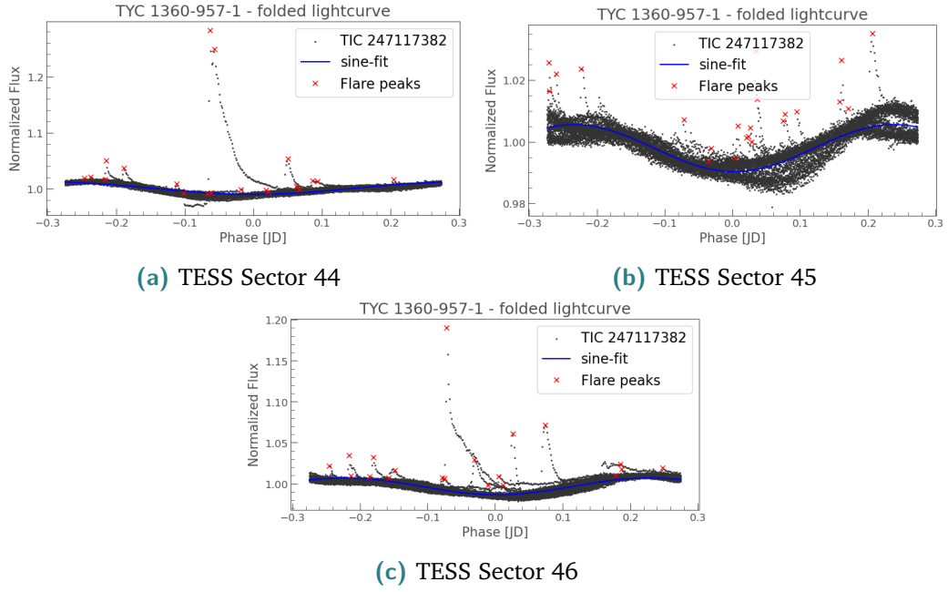
Fig. 4.20.: Folded lightcurves for TYC 1360-957-1. The blue lines shows the sine fits. The red crosses indicate the detected flare peaks.
