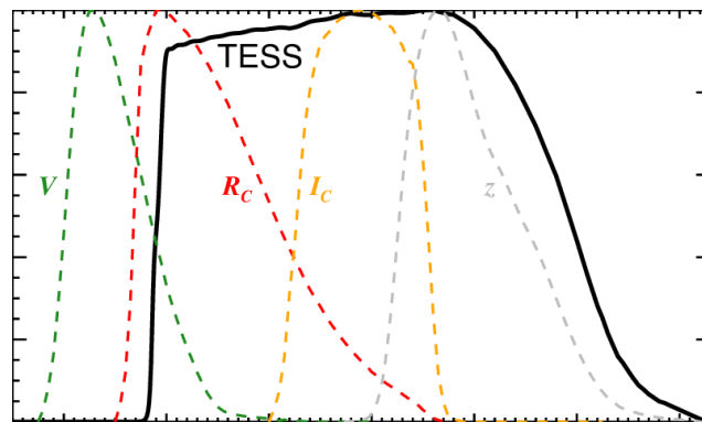
Fig. 1.6.: Johnson V, R_C , I_C and SDSS z (colored dashed lines) response curves and in comparison to TESS (solid black line). Image from Ricker et al. (2014b).
