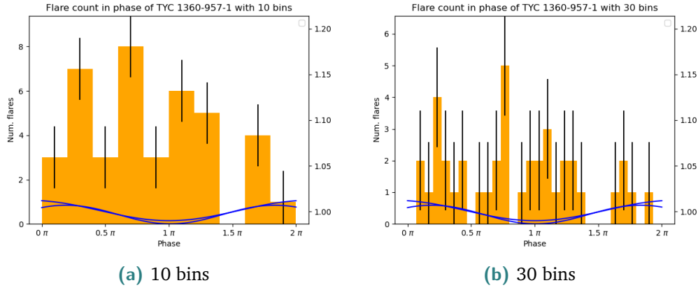
Fig. 4.18.: Histograms of TYC 1360-957-1 across the phase showing the number of flares in each bin. The error bar shows the standard deviation for the histogram. The blue lines show the various fits for the folded lightcurves used to generate the data, with the phase minimum at 1\pi and phase maximum at 0\pi/2\pi .
