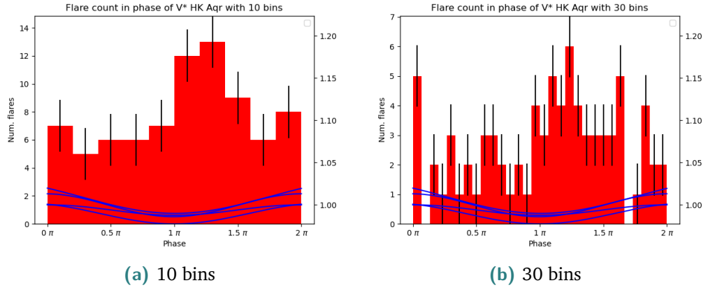
Fig. 4.25.: Histograms of V* HK Aqr across the phase showing the number of flares in each bin. The error bar shows the standard deviation for the histogram. The blue lines show the various fits for the folded lightcurves used to generate the data, with the phase minimum at 1\pi and phase maximum at 0\pi/2\pi .
