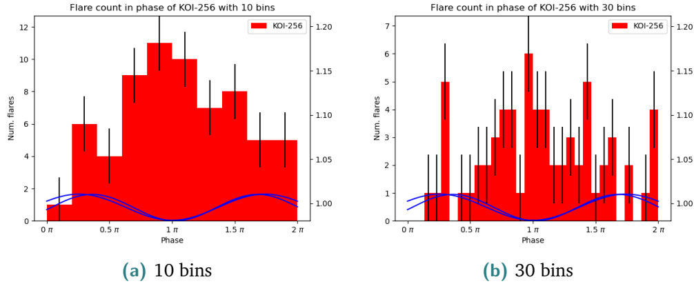
Fig. 4.31.: Histograms of KOI-256 across the phase showing the number of flares in each bin. The error bar shows the standard deviation for the histogram. The blue lines show the various fits for the folded lightcurves used to generate the data, with the phase minimum at 1\pi and phase maximum at 0\pi/2\pi .
