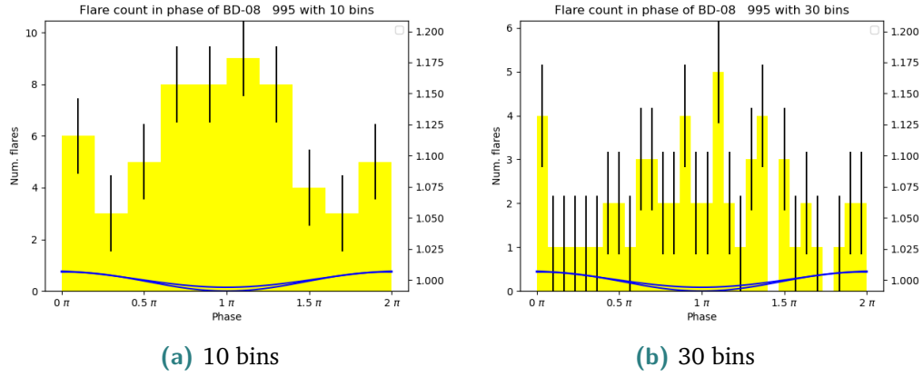
Fig. 4.15.: Histograms of BD-08 995 across the phase showing the number of flares in each bin. The error bar shows the standard deviation for the histogram. The blue lines show the various fits for the folded lightcurves used to generate the data, with the phase minimum at 1\pi and phase maximum at 0\pi/2\pi .
