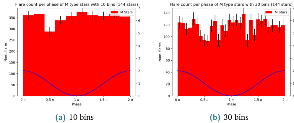
Fig. 4.1.: Histogram showing the amount of flares per phase for all 144 M dwarfs used in this study. The x-axis represents the normalized phase of the folded lightcurves. There are 10 bins (a)/30 bins (b) of the phase, showing the number of flares per bin. The error bar shows the standard deviation for the histogram. The blue line indicates an idealized phase (sine curve), with the maximum at phase 0\pi/2\pi and the minimum at phase 1\pi .
