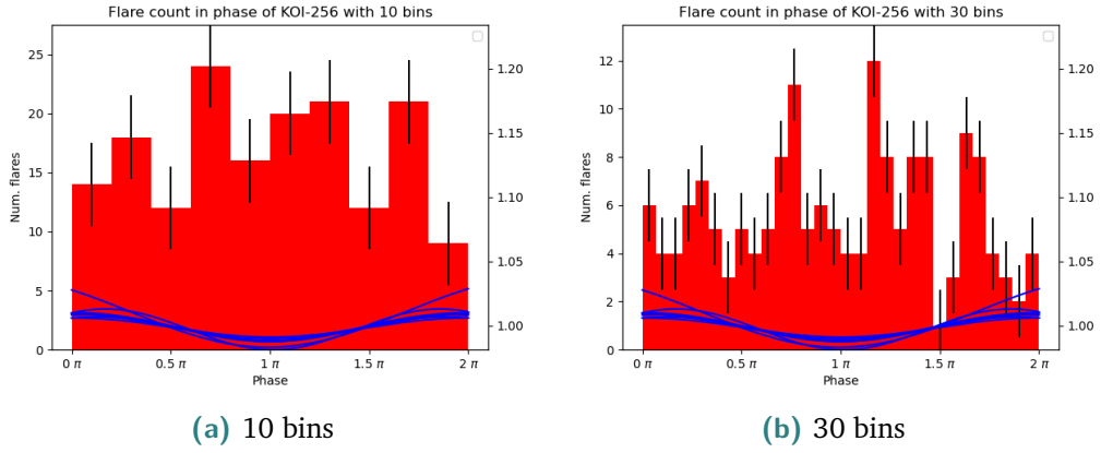
Fig. 4.30.: Histograms of KOI-256 across the phase showing the number of flares in each bin. The error bar shows the standard deviation for the histogram. The blue lines show the various fits for the folded lightcurves used to generate the data, with the phase minimum at 1\pi and phase maximum at 0\pi/2\pi .
