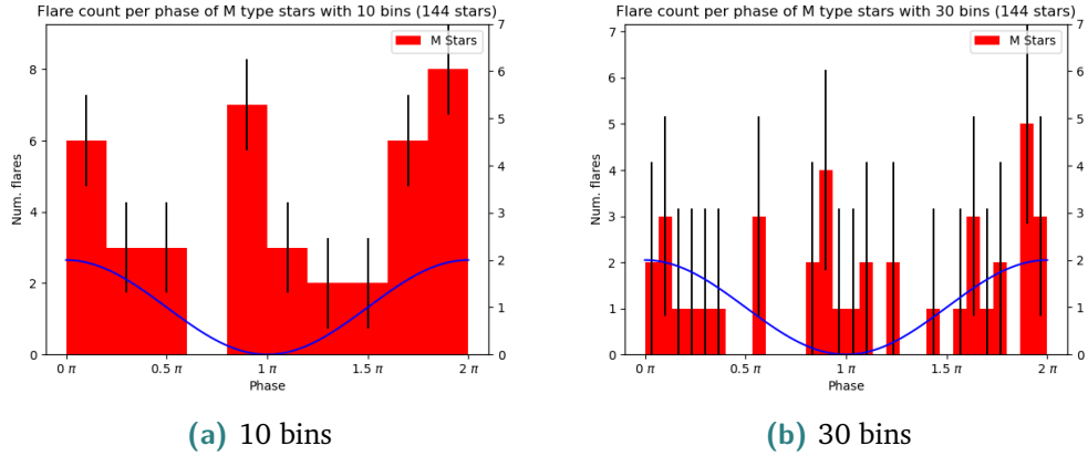
Fig. 4.3.: Histograms showing the amount of flares with a normalized peak of greater than 1.5 per phase for all 144 M dwarfs used in this study. The x-axis represents the normalized phase of the folded lightcurves. There are 10 (a) /30 (b) bins of the phase, showing the number of flares per bin. The error bar shows the standard deviation for the histogram. The blue line indicates an idealized phase (sine curve), with the maximum at phase 0\pi/2\pi and the minimum at phase 1\pi .
