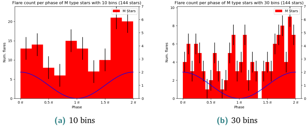
Fig. 4.2.: Histograms showing the amount of flares with a normalized peak of greater than 1.25 per phase for all 144 M dwarfs used in this study. The x-axis represents the normalized phase of the folded lightcurves. There are 10 (a) /30 (b) bins of the phase, showing the number of flares per bin. The error bar shows the standard deviation for the histogram. The blue line indicates an idealized phase (sine curve), with the maximum at phase 0\pi/2\pi and the minimum at phase 1\pi .
