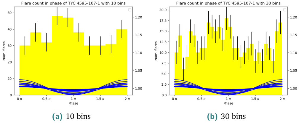
Fig. 4.21.: Histograms of TYC 4595-107-1 across the phase showing the number of flares in each bin. The error bar shows the standard deviation for the histogram. The blue lines show the various fits for the folded lightcurves used to generate the data, with the phase minimum at 1\pi and phase maximum at 0\pi/2\pi .
