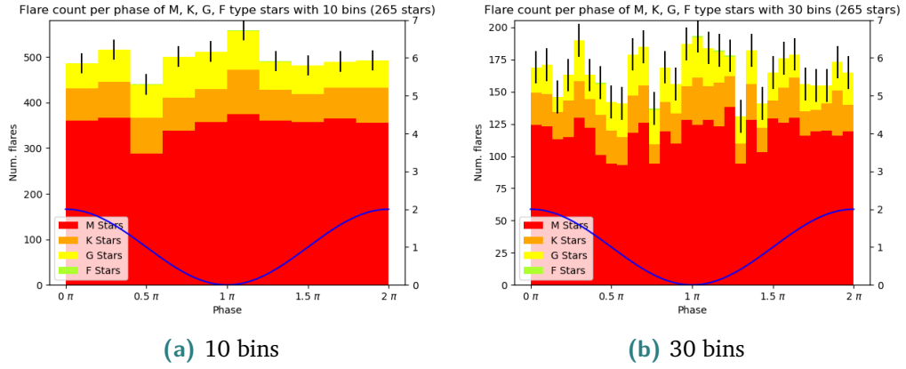
Fig. 4.14.: Histograms showing the amount of flares per phase for all 265 dwarfs used in this study. The x-axis represents the normalized phase of the folded lightcurves. There are 10 bins (a)/30 bins (b) of the phase, showing the number of flares per bin. The colors show the individual amount for each spectral type with the amount being stacked ontop of each other. The error bar shows the standard deviation for the histogram. The blue line indicates an idialized phase (sine curve), with the maximum at phase 0\pi/2\pi and the minimum at phase 1\pi .
