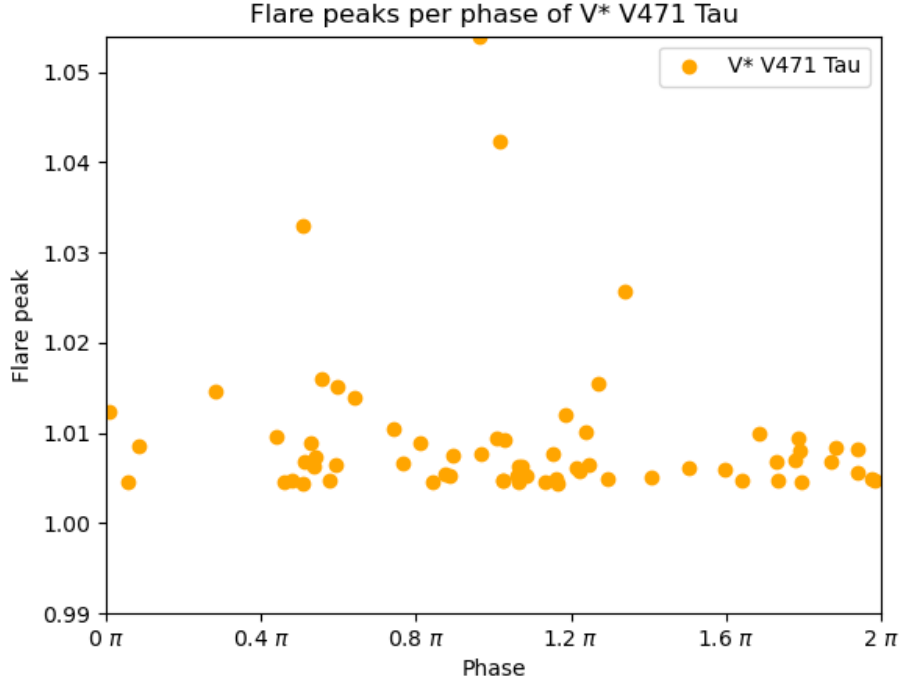
Fig. 4.24.: Distribution of flare peaks in relation to the normalized phase at which they occurred. Y-Axis shows the flare peak and is limited to the value of the highest peak detected. The x-axis shows the normalized phase.
