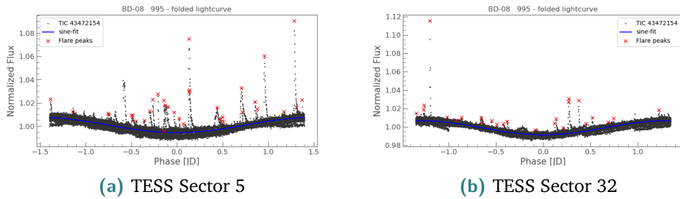
Fig. 4.17.: Folded lightcurves for BD-08 995. The blue lines shows the sine fits calculated. The red crosses indicate the detected flare peaks.
