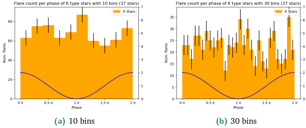
Fig. 4.9.: Histograms showing the amount of flares with a normalized peak of less than 1.05 per phase for all 37 K dwarfs used in this study. The x-axis represents the normalized phase of the folded lightcurves. There are 10 (a)/30 (b) bins of the phase, showing the number of flares per bin. The error bar shows the standard deviation for the histogram. The blue line indicates an idealized phase (sine curve), with the maximum at phase 0\pi/2\pi and the minimum at phase 1\pi .
