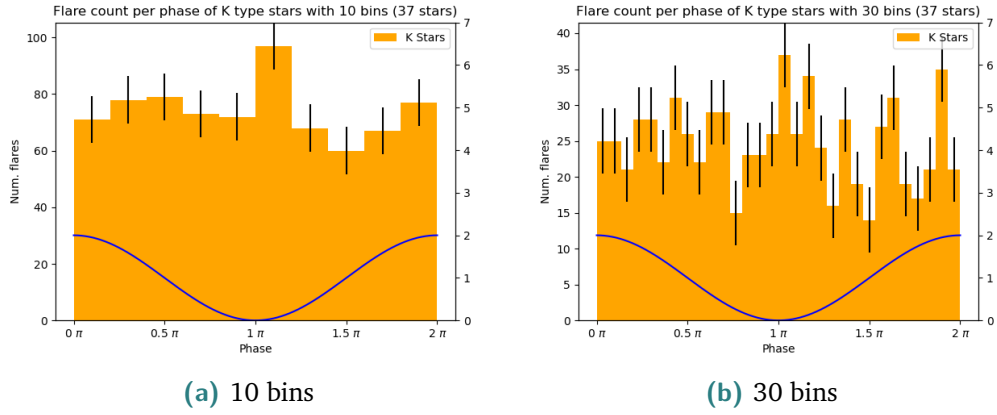
Fig. 4.6.: Histogram showing the amount of flares per phase for all 37 K dwarfs used in this study. The x-axis represents the normalized phase of the folded lightcurves. There are 10 bins (a)/30 bins (b) of the phase, showing the number of flares per bin. The error bar shows the standard deviation for the histogram. The blue line indicates an idealized phase (sine curve), with the maximum at phase 0\pi/2\pi and the minimum at phase 1\pi .
