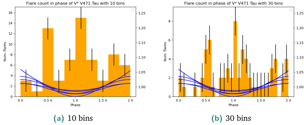
Fig. 4.22.: Histograms of V471 Tau across the phase showing the number of flares in each bin. The error bar shows the standard deviation for the histogram. The blue lines show the various fits for the folded lightcurves used to generate the data, with the phase minimum at 1\pi and phase maximum at 0\pi/2\pi .
