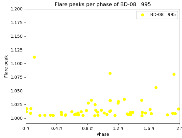
Fig. 4.16.: Distribution of flare peaks in relation to the normalized phase at which they occurred for BD-08 995. The y-axis shows the flare peak and the x-axis shows the normalized phase.
